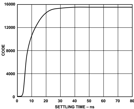
Figure 23. Settling Time
